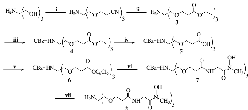
Scheme 2. Synthesis of trihydroxamate-containing amine 2 . Reagents and conditions: (i) \text{CH}_2=\text{CHCN} , aqueous KOH, dioxane; (ii) \text{H}_2\text{SO}_4 , ethanol, reflux; (iii) benzylchloroformate, \text{K}_2\text{CO}_3 , dioxane; (iv) 1 N aqueous NaOH, ethanol/water (7:3, v/v), 0 °C; (v) \text{C}_6\text{Cl}_5\text{OH} , DMAP, DCC, THF, 0 °C; (vi) \text{H}_2\text{NCHCONCH}_3\text{OH} , 11 \text{Et}_3\text{N} , THF, 25 °C; (vii) \text{H}_2/\text{Pd} , ethanol.
