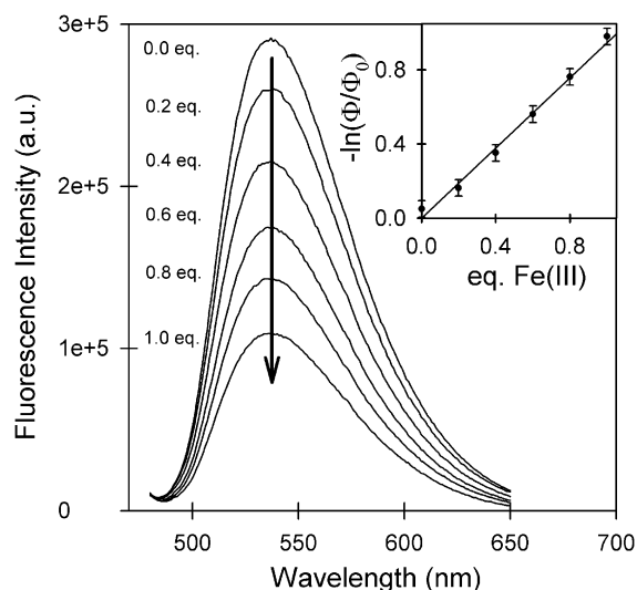
Figure 1. Fluorescence iron (III) titration curves with labelled ferrichrome analogue 1 . Aliquots of stock solutions of 1 in MeOH were treated with aliquots of methanolic solutions of \text{FeCl}_3 (0, 0.2, 0.4, 0.6, 0.8 and 1 equiv) and diluted with MeOH (80%)–0.1 N aqueous NaOAc (20%) to a final concentration of 5 \mu\text{M} .
