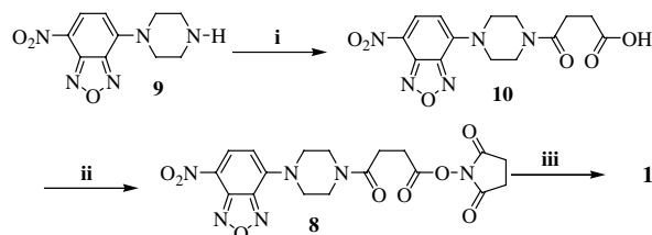
Scheme 3. Synthesis of NBD-ferrichrome analogue conjugate 1 . Reagents and conditions: (i) succinic anhydride, toluene/DMF (3:1, v/v), \Delta ; (ii) NHS, DCC, THF/DMF (4:3, v/v), 25 °C; (iii) 2 , THF/DMF (3:6, v/v), 25 °C.
